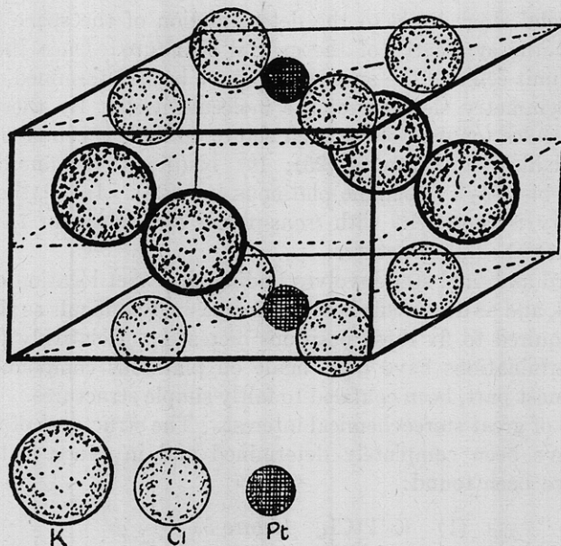
FIG. 5. The structure of K_2[PtCl_4]
