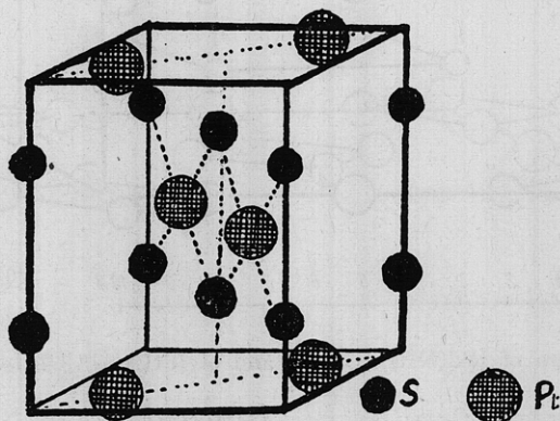
FIG. 8. The structure of PtS
